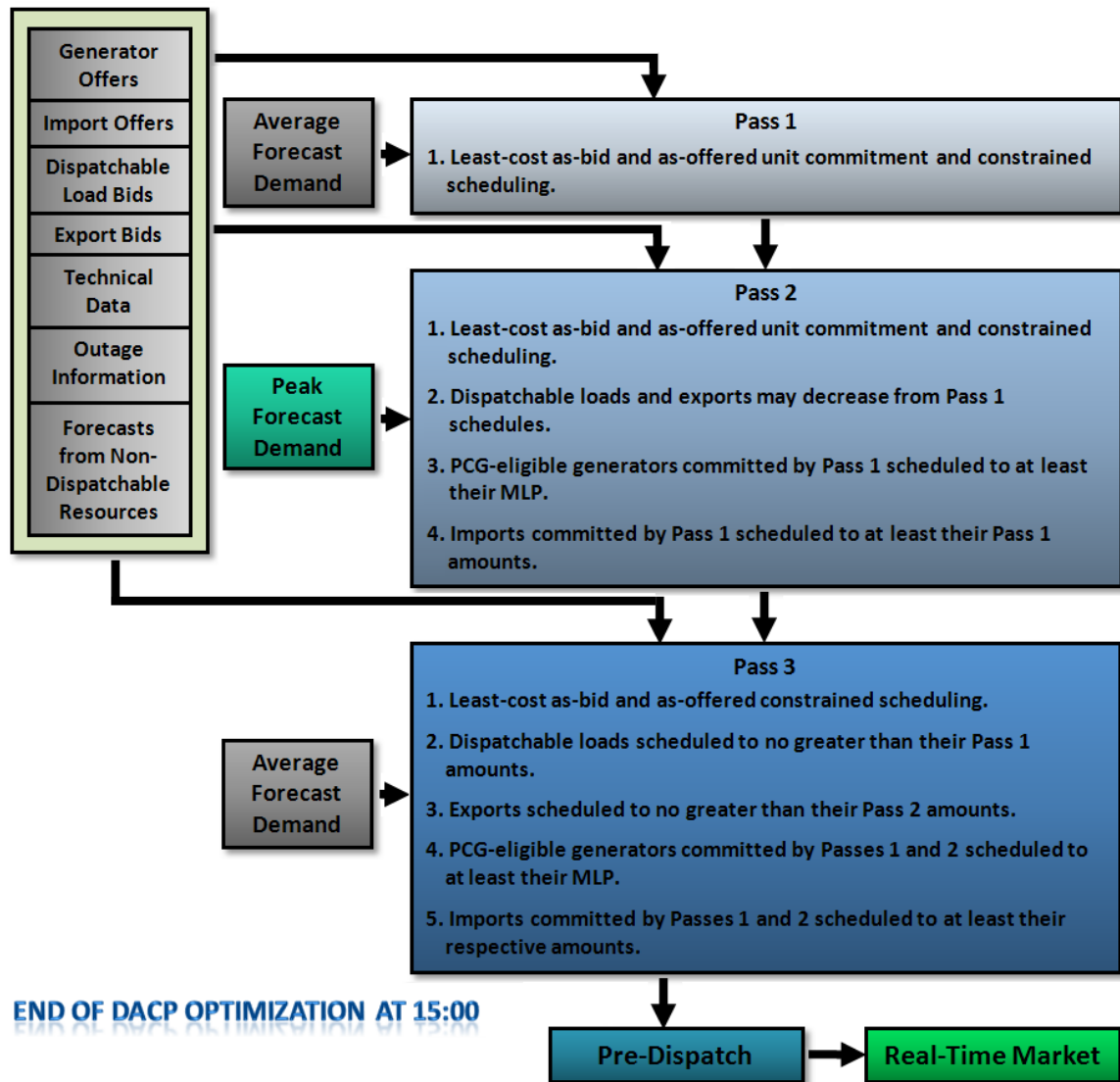
Figure 13: Three Passes of Constrained Algorithm
