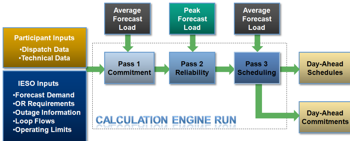
Figure 11: Day-Ahead Calculation Engine (DACE)
