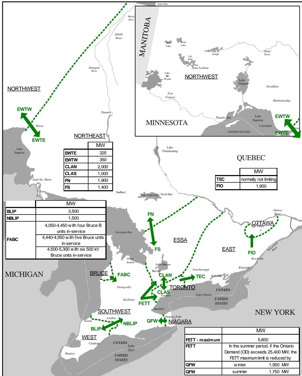
Figure 2.1.1 Ontario's Major Internal Transfer Interfaces
