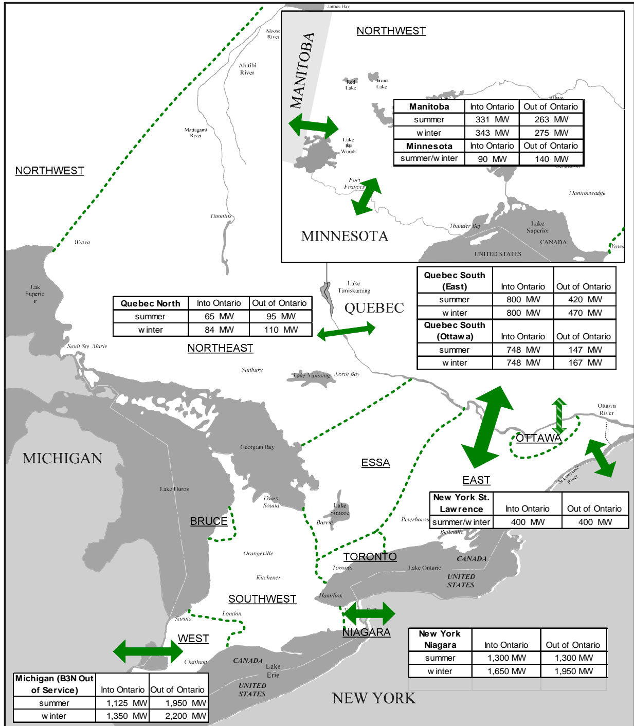
Figure 2.1.2 Ontario's Points of Interconnection with Neighbouring Areas
